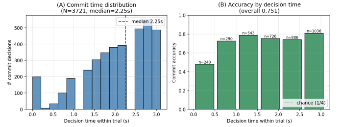
Fig. 8. When the selective decoder commits within a trial, pooled across 9 BCI-IV-2a subjects \times 5 seeds \times 2 configs ( N=3721 commit decisions); median decision time 2.25 s ( \sim 56\% of full trial length). (A) Commit-time distribution is bimodal: \sim 6\% of decisions fire immediately at the first step (impulsive-commit mode), the bulk ( \sim 85\% ) cluster between 1.25–3.0 s as the 140e head accumulates evidence, and very few fire in the 0.5–1.0 s window. (B) Commit accuracy by decision-time bin: early-impulse commits ( \leq 0.5 s) drop to 0.48, while every later bin ( \geq 1 s) is above 0.73, the expected speed-accuracy trade-off. Overall pooled commit accuracy 0.751.
