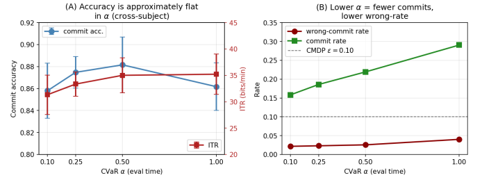
Fig. 5. CVaR \alpha sensitivity on the canonical 3-subject BCI-IV-2a panel (3 subj \times 5 seeds, eval-time sweep over a single distributional-CQL+CMDP \epsilon = 0.10 training). (A) Commit accuracy (blue) and ITR (red) are approximately flat in \alpha . (B) Wrong-commit rate (dark red, 0.022 \rightarrow 0.040 ) and commit rate (green, 0.16 \rightarrow 0.29 ) both double from \alpha = 0.10 to \alpha = 1.00 . The CMDP constraint ( \epsilon = 0.10 , dashed) is comfortably satisfied at every \alpha . \alpha is therefore an operating-point knob, not a no-op.
