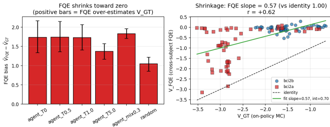
Fig. 7. Fitted-Q estimator shrinks toward zero on the N=9 LOSO OPE corpus. Linear fit V_{FQE} = 0.57 V_{GT} + 0.70 ( r = +0.62 ); weak-decodability subjects (red) exhibit 44% larger shrinkage.
