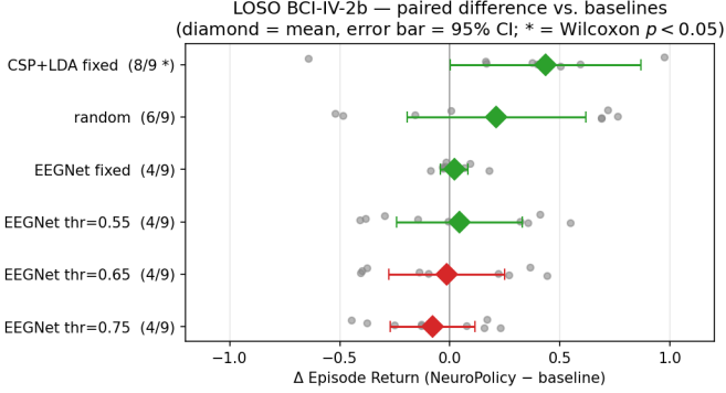
Fig. 4. Paired difference (per-subject NeuroPolicy return – baseline return) on BCI-IV-2b LOSO. Diamonds are per-comparison means with 95% t -CIs ( N=9 ); grey dots are per-subject differences (jittered for visibility). NeuroPolicy significantly beats CSP+LDA fixed-window ( p=0.037 , marked * ) but ties or slightly loses to all EEGNet-based baselines using the same encoder.
