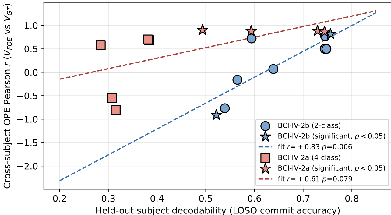
Cross-subject OPE calibration tracks decodability
