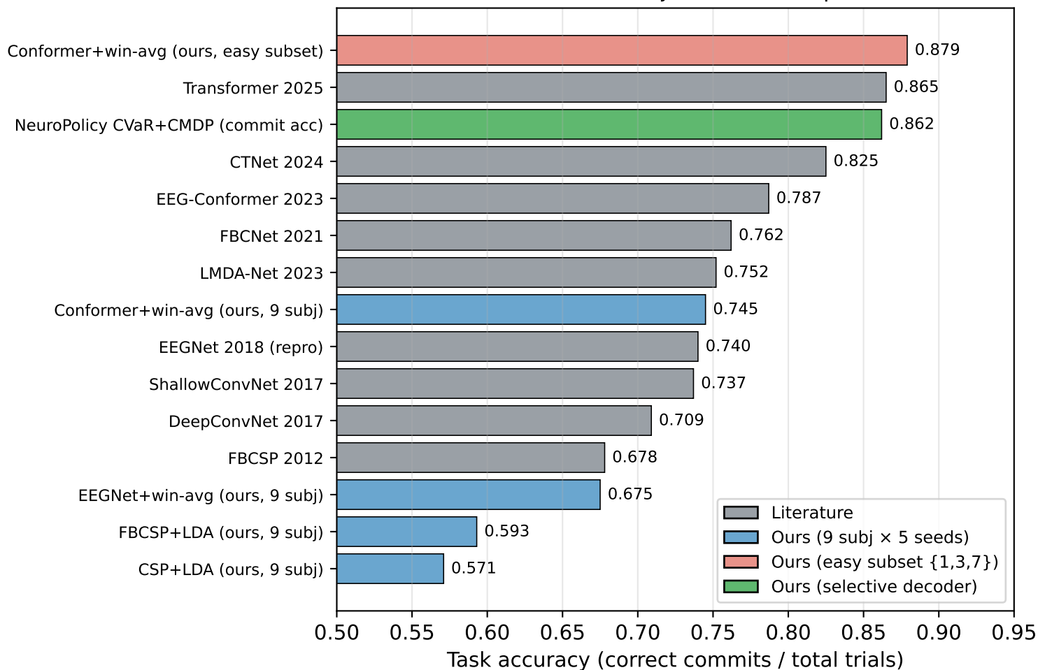
BCI-IV-2a 4-class within-subject canonical protocol (T → E)
