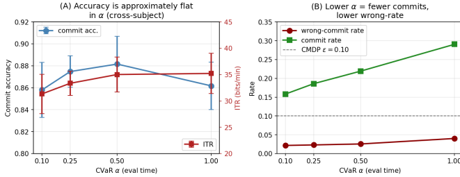
Fig. 5. CVaR \alpha sensitivity on the canonical 3-subject BCI-IV-2a panel (3 subj \times 5 seeds, eval-time sweep over a single distributional-CQL+CMDP \epsilon=0.10 training). (A) Commit accuracy (blue) and ITR (red) are approximately flat in \alpha . (B) Wrong-commit rate (dark red, 0.022 \rightarrow 0.040) and commit rate (green, 0.16 \rightarrow 0.29) both double from \alpha=0.10 to \alpha=1.00 . The CMDP constraint ( \epsilon=0.10 , dashed) is comfortably satisfied at every \alpha . \alpha is therefore an operating-point knob, not a no-op.
