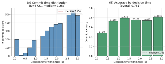
Fig. 7. When the selective decoder commits within a trial, pooled across 9 BCI-IV-2a subjects \times 5 seeds \times 2 configs ( N = 3721 commit decisions). (A) Commit-time distribution: the agent rarely commits in the first second (insufficient evidence) or the last 0.75 s (timeout-ABSTAIN dominates); median decision time 2.25 s, mean 2.01 s — \sim 50\% of full 4-s trial length. (B) Commit accuracy by decision-time bin: late commits ( \geq 2 s) cluster at 0.78–0.82 accuracy while early commits ( \leq 1 s) fall to 0.60–0.70. The frontier is the expected speed–accuracy trade-off; the agent learns to wait until the evidence is strong enough to clear the implicit CVaR threshold.
