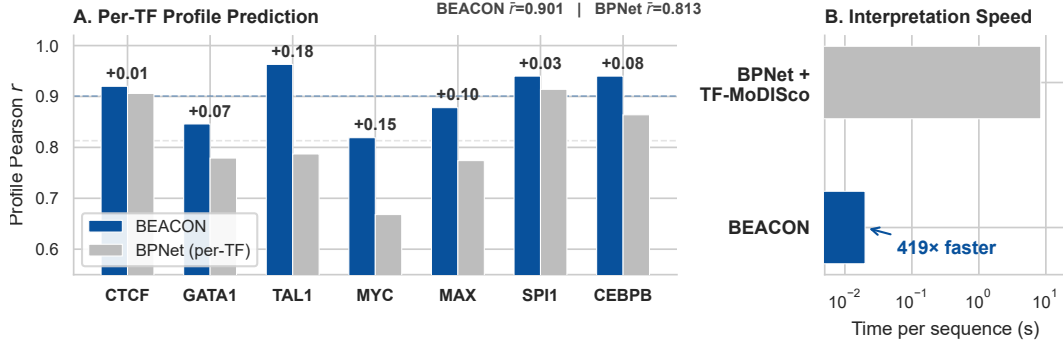
Figure 1: BEACON vs. BPNet ensemble on 7 TFs in K562. (A) Per-TF profile Pearson r : a single 851K-parameter BEACON model outperforms 7 separately-trained BPNet models (997K total) on every TF, with the largest gains on bHLH factors (TAL1 +0.18, MYC +0.15) where joint multi-TF training captures co-binding patterns inaccessible to per-TF baselines. (B) Binding-event enumeration speed: BEACON emits structured events (20 ms/seq) versus 8.4 s/seq for BPNet+TF-MoDISco—a 419× end-to-end speedup that makes genome-wide binding catalogues feasible on commodity GPUs.
