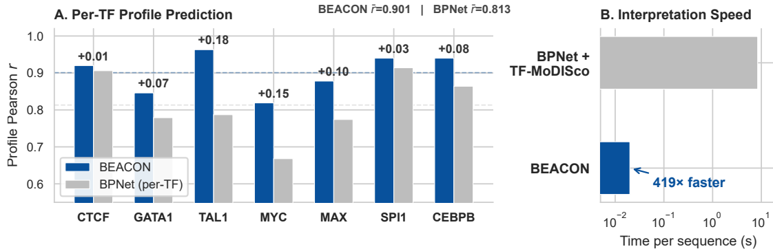
Figure 1: BEACON vs. BPNet on 7 TFs in K562. (A) Per-TF profile Pearson r : a single BEACON model (850K params) outperforms 7 separately trained BPNet models (997K total params) on every TF. Dashed lines show mean r across TFs ( \bar{r} = 0.901 for BEACON vs. \bar{r} = 0.813 for BPNet). The largest improvements occur on bHLH factors (TAL1: +0.18, MYC: +0.15), where BEACON’s joint multi-TF architecture captures cooperative binding patterns—such as obligate MYC–MAX heterodimerization—that are inaccessible to per-TF models. (B) Binding site enumeration speed: BEACON directly outputs structured binding events (position, identity, confidence) in 20 ms per sequence, compared to 8.4 s for BPNet followed by TF-MoDISco post-hoc attribution—a 419 \times speedup that enables genome-wide binding catalogues in minutes rather than hours.
