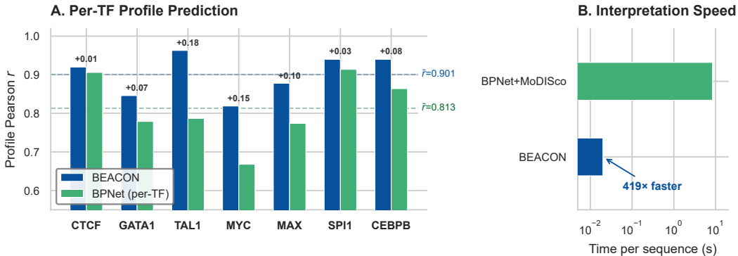
Figure 1: BEACON vs. BPNet ensemble on 7 TFs in K562. (A) Per-TF profile Pearson r : a single 851K-parameter BEACON model outperforms 7 separately-trained BPNet models (997K total) on every TF, with the largest gains on bHLH factors (TAL1 +0.18, MYC +0.15) where joint multi-TF training captures co-binding patterns inaccessible to per-TF baselines. (B) Binding-event enumeration speed: BEACON emits structured events (20 ms/seq) versus 8.4 s/seq for BPNet+TF-MoDISco—a 419 \times end-to-end speedup that makes genome-wide binding catalogues feasible on commodity GPUs.
