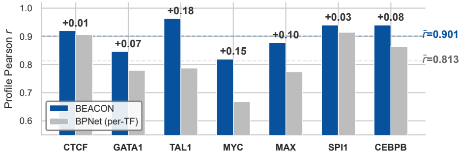
A. Per-TF Profile Prediction
