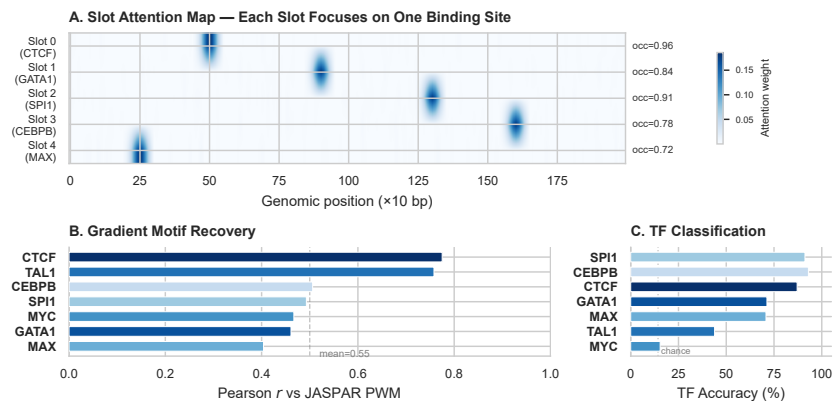
Figure 2: Interpretable binding event decomposition. (A) Slot attention maps for an example locus containing 5 binding sites: each slot focuses sharply on a single binding event, with occupancy scores ( occ ) reflecting binding confidence. Slots self-organize to cover distinct genomic positions without supervision. (B) Gradient-derived per-slot motifs correlate with canonical JASPAR position weight matrices (5/7 TFs achieve r > 0.50 ), confirming that slots learn biologically meaningful sequence features. CTCF ( r = 0.78 ) and TAL1 ( r = 0.76 ) show the strongest recovery. (C) Per-TF classification accuracy via Hungarian matching: SPI1 and CEBPB exceed 90%, while bHLH factors (MYC, TAL1) are harder to discriminate due to shared E-box binding preferences.
