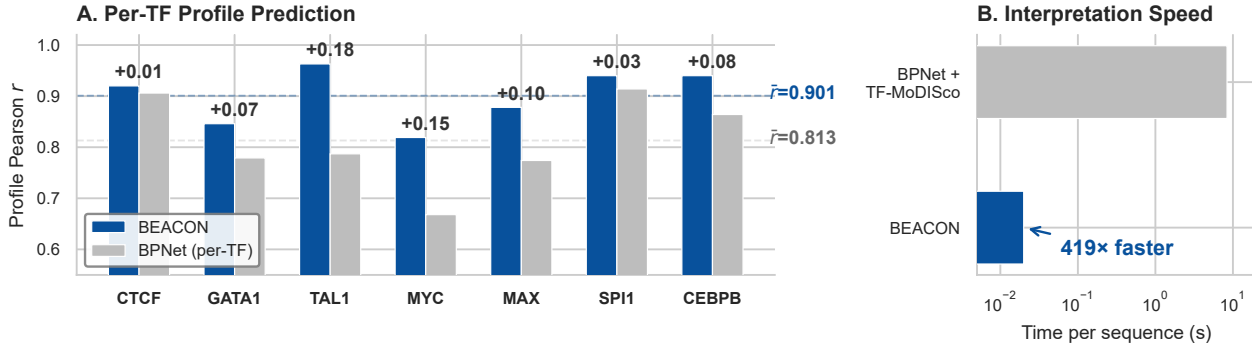
Figure 1: BEACON vs. BPNet on 7 TFs in K562. (A) Per-TF profile Pearson r : a single BEACON model (850K params) outperforms 7 separately trained BPNet models (997K total params) on every TF, with the largest improvements on bHLH factors (TAL1: +0.18, MYC: +0.15) where multi-TF modeling captures co-binding patterns inaccessible to per-TF models. (B) Binding site enumeration speed: BEACON directly outputs binding events in 20 ms per sequence, compared to 8.4 s for BPNet followed by TF-MoDISco post-hoc attribution—a 419 \times speedup that enables genome-wide analysis in minutes rather than hours.
