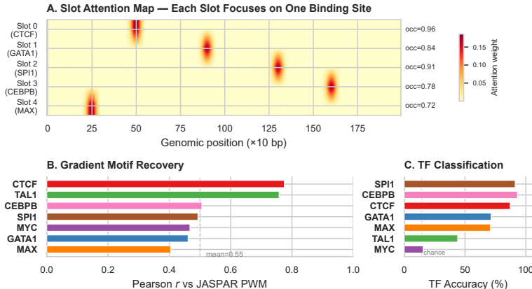
Figure 2: Interpretable binding event decomposition. (A) Slot attention maps for an example locus containing 5 binding sites: each slot focuses sharply on a single binding event, with occupancy scores ( occ ) reflecting binding confidence. Slots self-organize to cover distinct genomic positions without supervision. (B) Gradient-derived per-slot motifs correlate with canonical JASPAR position weight matrices (5/7 TFs achieve r>0.50 ), confirming that slots learn biologically meaningful sequence features. CTCF ( r=0.78 ) and TAL1 ( r=0.76 ) show the strongest recovery. (C) Per-TF classification accuracy via Hungarian matching: SPI1 and CEBPB exceed 90%, while bHLH factors (MYC, TAL1) are harder to discriminate due to shared E-box binding preferences.
