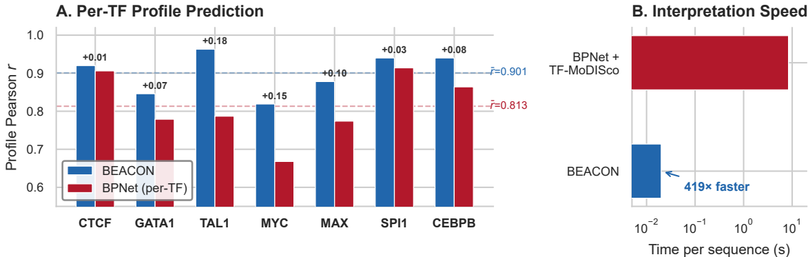
Figure 1: BEACON vs. BPNet on 7 TFs in K562. (A) Per-TF profile Pearson r : a single BEACON model (850K params) outperforms 7 separately trained BPNet models (997K total params) on every TF, with the largest improvements on bHLH factors (TAL1: +0.18, MYC: +0.15) where multi-TF modeling captures co-binding patterns inaccessible to per-TF models. (B) Binding site enumeration speed: BEACON directly outputs binding events in 20 ms per sequence, compared to 8.4 s for BPNet followed by TF-MoDISco post-hoc attribution—a 419 \times speedup that enables genome-wide analysis in minutes rather than hours.
