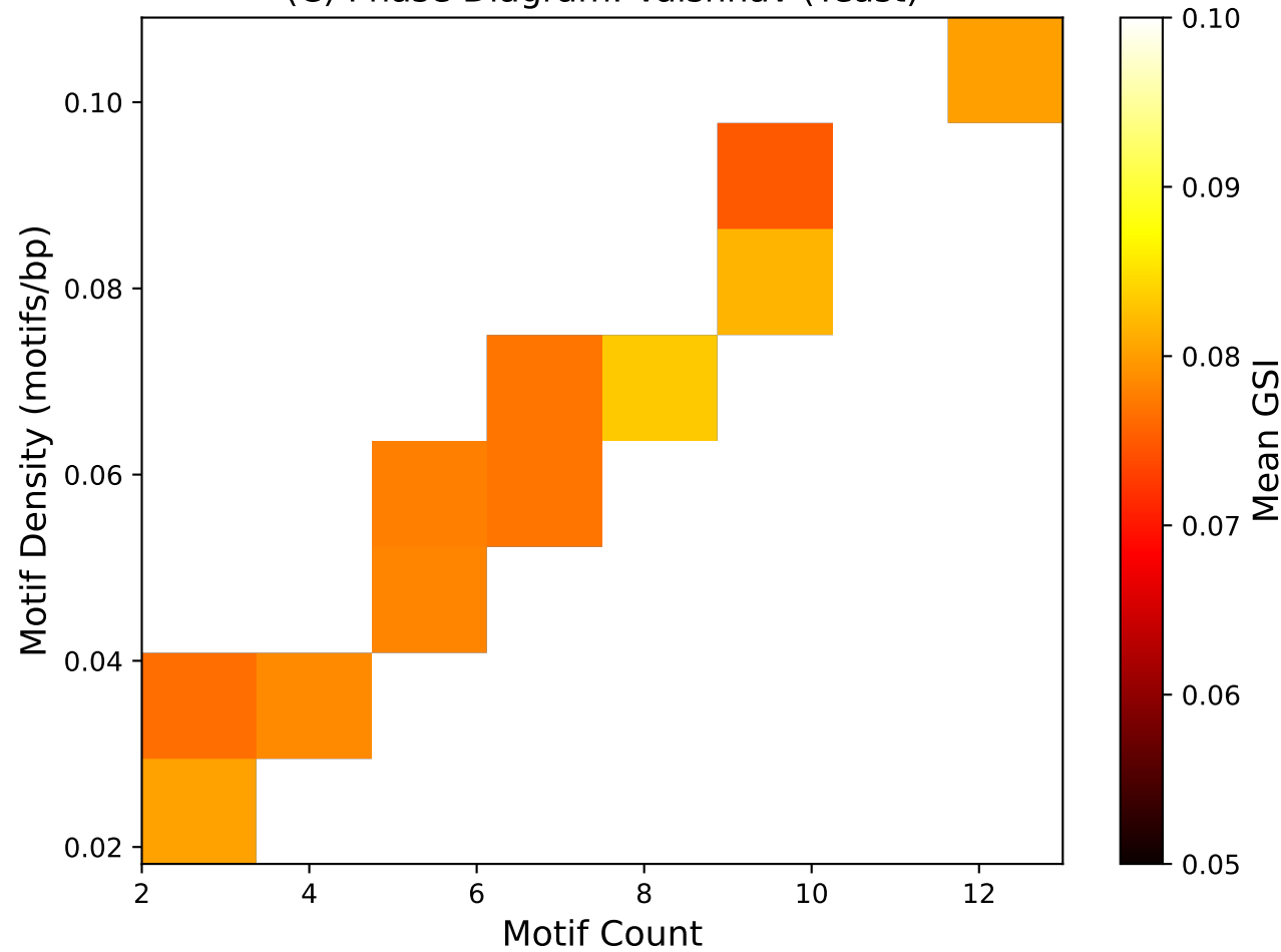
(C) Phase Diagram: Vaishnav (Yeast)
