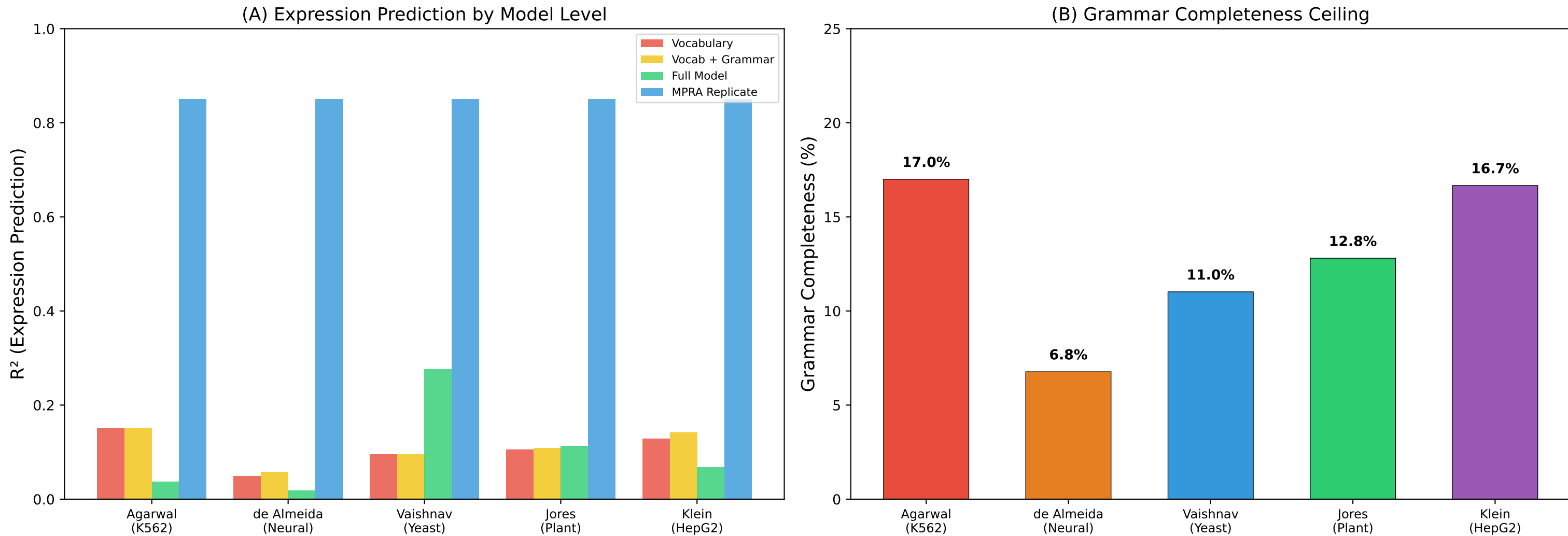
Figure 6: Grammar Completeness Ceiling
