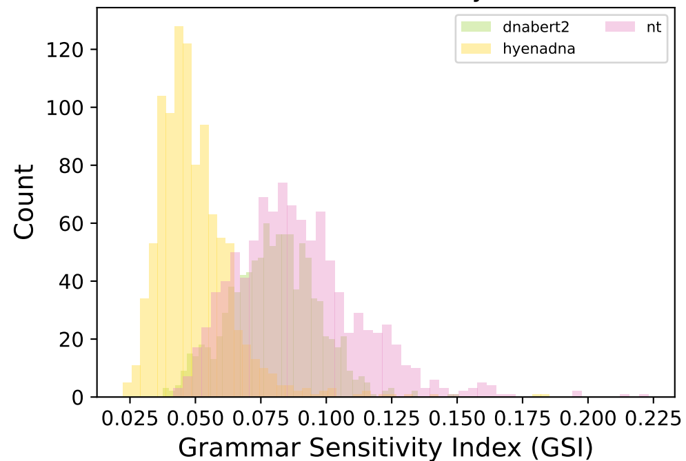
(A) GSI Distribution by Model
