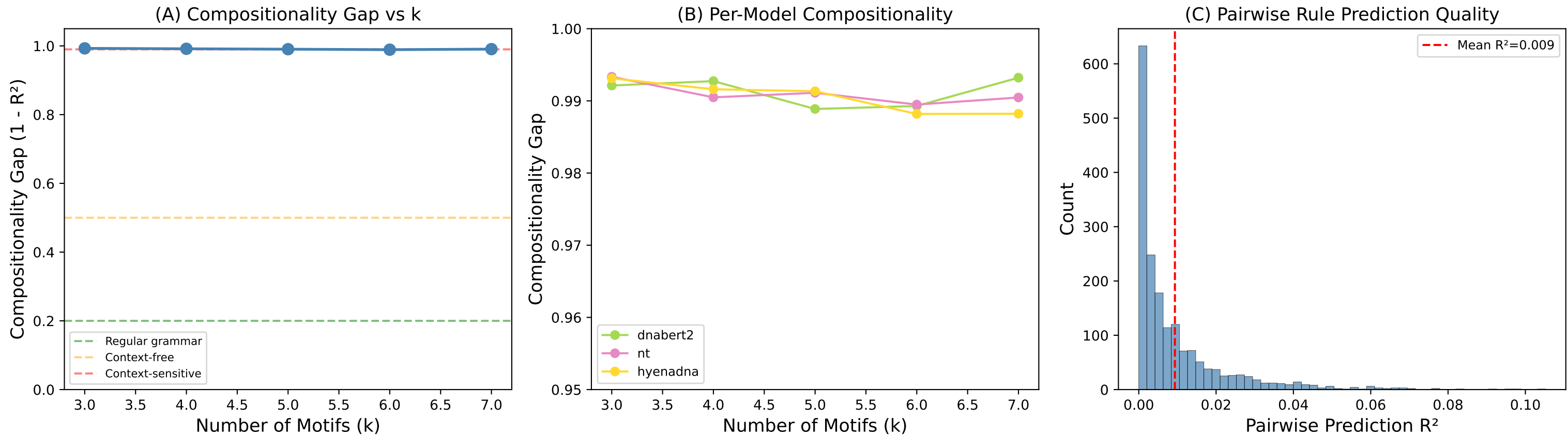
Figure 2: Compositionality & Chomsky Classification
