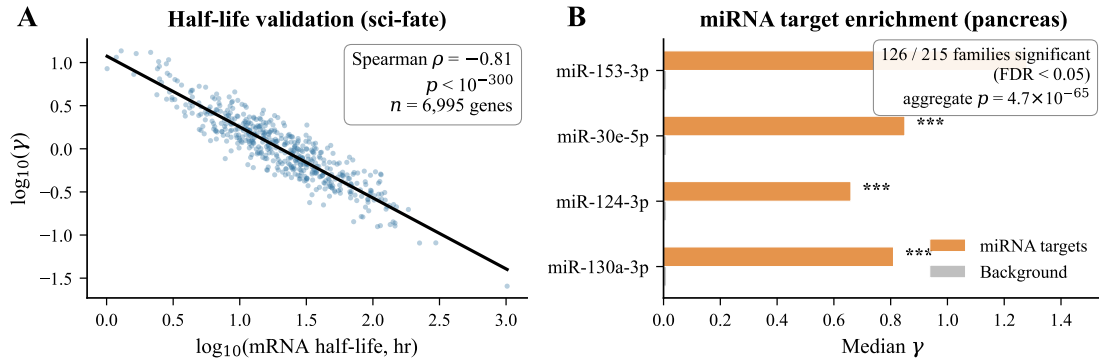
Figure 2: Validation of \gamma estimates. (A) Per-gene median \gamma correlates strongly with published mRNA half-lives in the sci-fate metabolic-labeling dataset (Spearman \rho = -0.81 ; correlations of -0.35 to -0.40 in 10x developmental datasets). (B) miRNA targets show significantly elevated \gamma relative to non-target background genes in the pancreas dataset (126/215 families significant at FDR < 0.05 ; aggregate p = 4.7 \times 10^{-65} ).
