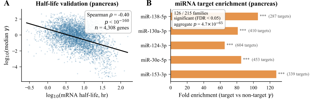
Figure 2: Validation of per-cell \hat{\gamma} . (A) Per-gene median \hat{\gamma} vs. published half-lives. scPTR achieves Spearman \rho = -0.81 on sci-fate, \rho = -0.40 on pancreas, outperforming scVelo ( -0.37 ) and velVI ( -0.28 ). (B) miRNA target enrichment: 59% of 215 TargetScan 8.0 families are significant at \text{FDR} < 0.05 ; aggregate p = 4.7 \times 10^{-65} .
