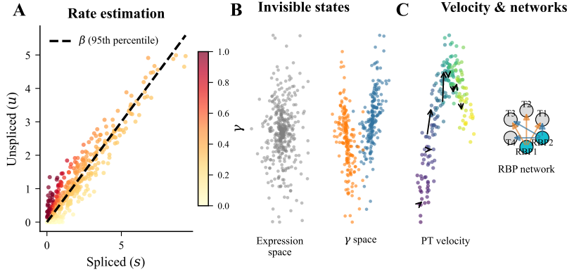
Figure 1: scPTR framework. (A) Gene-specific splicing rates ( \beta ) are estimated via quantile regression on unspliced/spliced phase portraits; per-cell degradation rates are then computed as \gamma = \beta \cdot u/s after k -NN Gaussian-kernel smoothing. (B) Clustering in \gamma -space via PCA and Leiden community detection reveals post-transcriptional states that are invisible to standard expression-based analysis. (C) Post-transcriptional velocity (the neighbor-averaged \gamma gradient) captures degradation dynamics orthogonal to RNA velocity, while library-size-corrected elastic net regression infers RBP–target regulatory networks.
