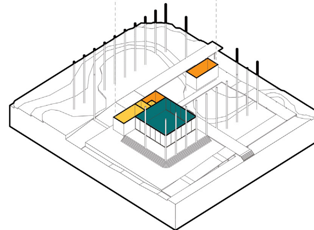
■ steel columns ■ reinforced concrete shear walls
