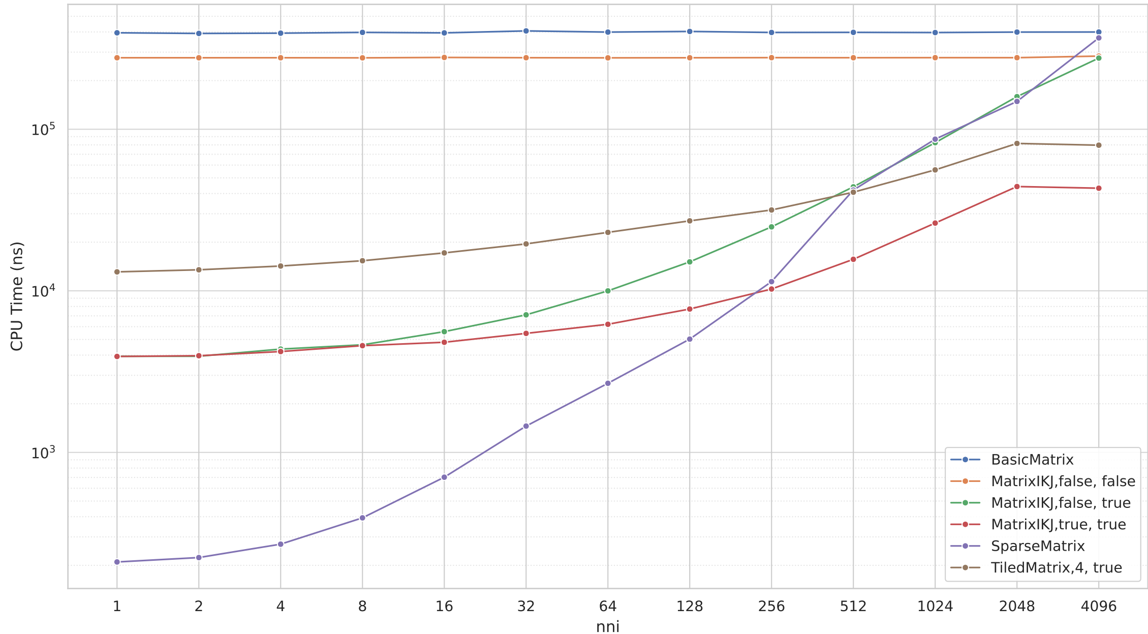
Matrix Multiplication Performance vs. NNI (Size 64)
