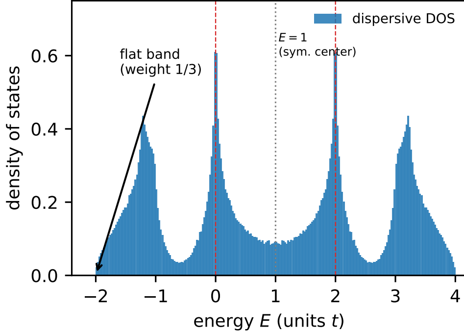
FIGURE 1. Density of states of the hyperkagome tight-binding model ( t = 1 ). Four flat bands at E = -2 carry weight 1/3 ; the eight dispersive bands fill [-2, 4] and are exactly symmetric about E = 1 , with principal van Hove singularities at E = 0, 2 (dashed) and weaker interior features at E = -1, 3 and E = 1 \pm \sqrt{5} (see text).
