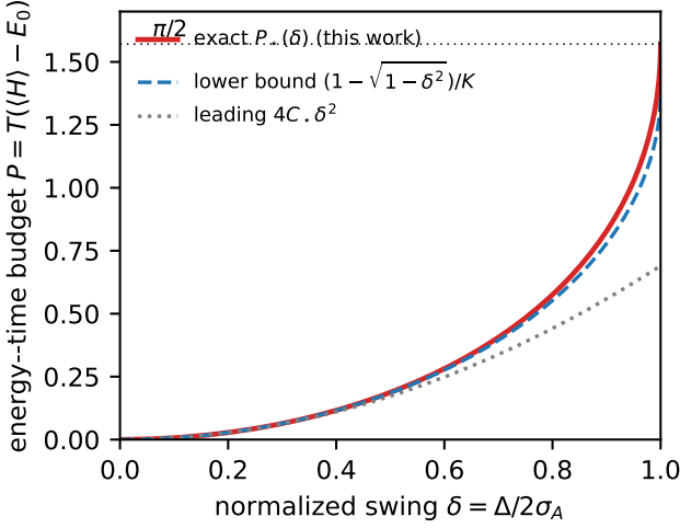
FIG. 2. The exact observable trade-off curve P_*(\delta) , Eq. (6): the minimum energy-time budget P = T(\langle H \rangle - E_0) for a normalized swing \delta = \Delta/2\sigma_A , tight at every \delta . Its slope as \delta \rightarrow 0 is set by C_* and its \delta \rightarrow 1 limit is \pi/2 . It lies above the elementary lower bound (1 - \sqrt{1 - \delta^2})/K and its leading term 4C_*\delta^2 .
