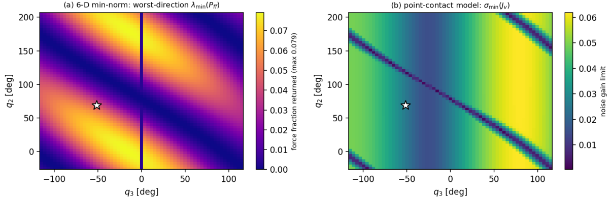
FIGURE 2. Force estimation over a slice of the workspace ( q_1 = 0 , q_4 = 0.4 rad). (a) Worst-direction eigenvalue of P_H at the unweighted-SI baseline, the fraction of a pure contact force that the six-dimensional inversion returns as force. Note the scale: it never exceeds 0.079 anywhere on the slice, so even the most favorable posture returns under a twelfth of a push along that direction, and the pattern is a property of the geometry rather than of any one configuration. This is the effect that has been misread as blindness of the mechanism. (b) \sigma_{\min}(J_v) , which bounds noise amplification for the point-contact inversion and is the quantity that actually limits it. The star marks the task configuration.
