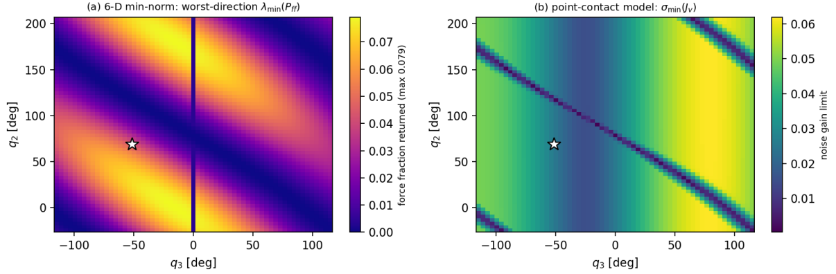
FIGURE 2. Force estimation over a slice of the workspace ( q_1 = 0 , q_4 = 0.4 rad). (a) Worst-direction eigenvalue of P_{ff} at the unweighted-SI baseline, the fraction of a pure contact force that the six-dimensional inversion returns as force. Note the scale: it never exceeds 0.079 anywhere on the slice, so even the most favorable posture returns under a twelfth of a push along that direction, and the pattern is a property of the geometry rather than of any one configuration. This is the effect that has been misread as blindness of the mechanism. (b) \sigma_{\min}(J_v) , which bounds noise amplification for the point-contact inversion and is the quantity that actually limits it. The star marks the task configuration.
