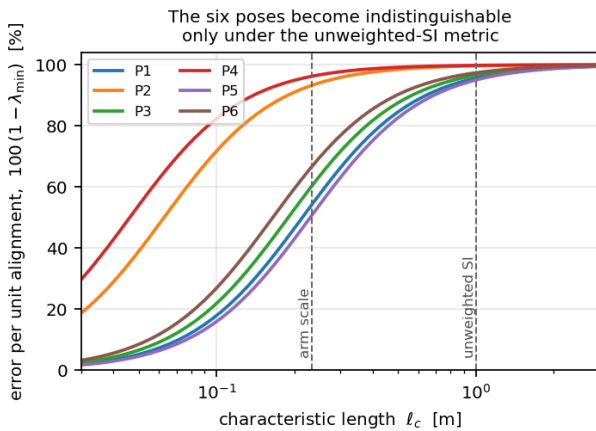
FIGURE 3. The slope of (13), 1 - \lambda_{\min} , against the characteristic length, at the six configurations of the directional sweep. Each pose has its own slope at small \ell_c and all six approach a common value as \ell_c grows, so at the unweighted-SI baseline they are nearly indistinguishable while at the scale of the arm they are not. This is what the pooled correlation of 0.9993 measures and what it conceals. The direction that is lost is the same throughout, by Proposition 3, and it is only the slope that moves.
