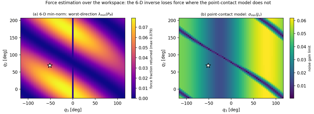
FIGURE 2. Force estimation over a slice of the workspace ( q_1 = 0 , q_4 = 0.4 rad). (a) Worst-direction eigenvalue of P_H at the unweighted-SI baseline, the fraction of a pure contact force that the six-dimensional inversion returns as force. Note the scale: it never exceeds 0.079 anywhere on the slice, so even the most favorable posture returns under a twelfth of a push along that direction, and the pattern is a property of the geometry rather than of any one configuration. This is the effect that has been misread as blindness of the mechanism. (b) \sigma_{\min}(J_v) , which bounds noise amplification for the point-contact inversion and is the quantity that actually limits it. The star marks the task configuration.
