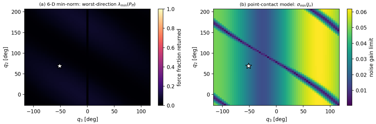
FIGURE 2. Force estimation over a slice of the workspace ( q_1 = 0 , q_4 = 0.4 rad). (a) Worst-direction eigenvalue of P_{ff} , the fraction of a pure contact force that the six-dimensional inversion returns as force; close to zero throughout, which is the effect that has been misread as blindness of the mechanism. (b) \sigma_{\min}(\mathbf{J}_v) , which bounds noise amplification for the point-contact inversion and is the quantity that actually limits it. The star marks the task configuration.
