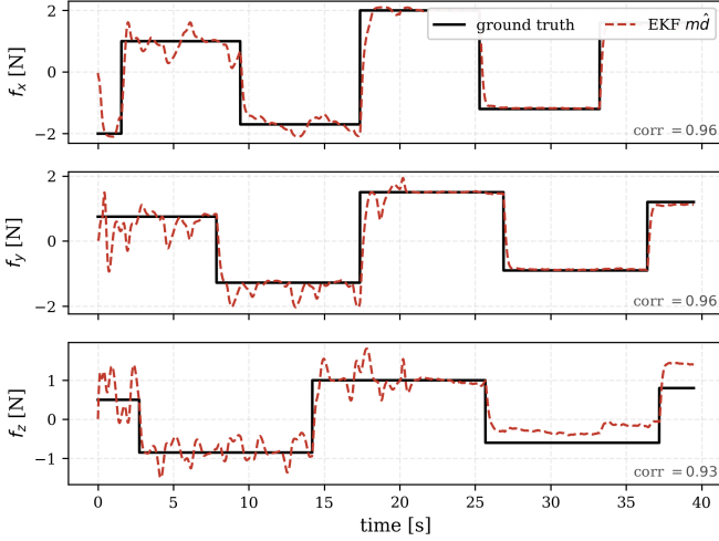
Fig. 2. Virtual force sensor in the time domain (single representative run): the EKF estimate (the specific force \hat{\mathbf{d}} scaled by the mass to newtons) tracks the applied wind steps on all three axes.
