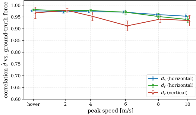
Fig. 3. Per-axis force correlation against excitation ( N=10 ; 9 in hover). All axes read accurately (0.91–0.98, step ground truth); d_z stays high in hover because the held mass absorbs the m – d_z ambiguity of Proposition 1.
