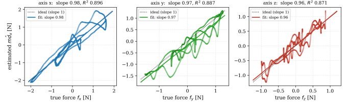
Fig. 4. Calibration curve of the virtual force sensor: estimated force m\hat{\mathbf{d}} versus the applied force, per axis, under a sinusoidal wind. The near-unity slope and high R^2 show the IMU-residual reading is a well-calibrated force measurement.
