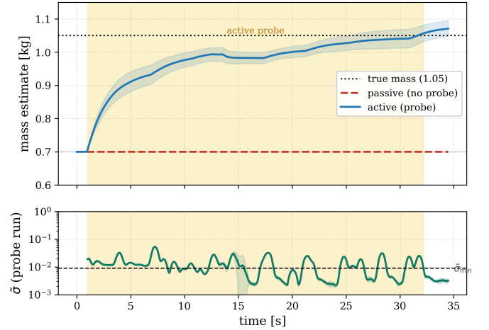
Fig. 8. Mass recovery from a wrong hover prior (0.70 kg), N=5 , mean \pm std. Passively the estimate stays frozen; the active probe (shaded) lifts \tilde{\sigma} above the threshold (bottom), recovers the mass, then withdraws.
