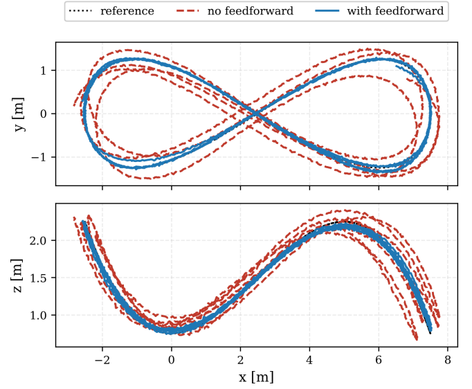
Fig. 10. Trajectory under wind, orthogonal projections sharing the x axis. With the estimated-force feedforward (blue) the vehicle stays on the reference (dotted); without it (red) the wind pushes it off the path.
