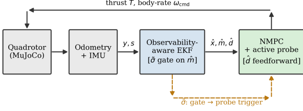
Fig. 1. Architecture of the self-calibrating virtual force sensor. The EKF outputs the external force \hat{d} , the mass calibration \hat{m} , and the identifiability \tilde{\sigma} , which gates the calibration and triggers the active probe; the NMPC (application) feeds \hat{d} forward.
