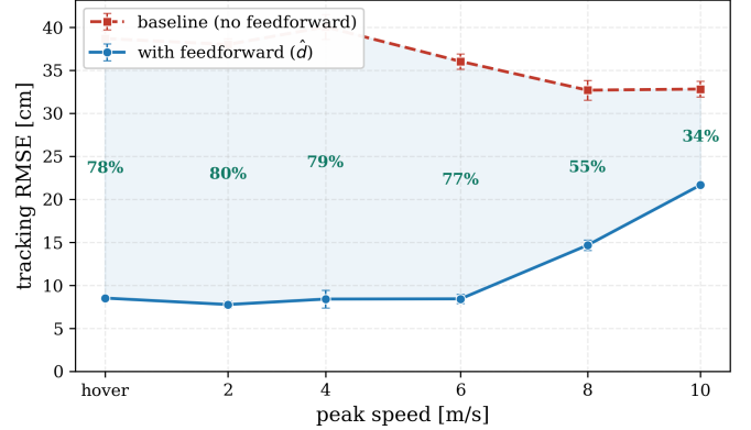
Fig. 11. Disturbance rejection against speed ( N = 5 per mode; hover N = 4 , mean \pm std). Feeding the estimated force to the controller reduces the tracking error most when the wind dominates (hover) and less as the speed grows.
