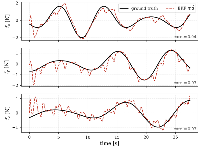
Fig. 12. Virtual force sensor under a sinusoidal wind (single representative run), a different disturbance profile from the steps of Fig. 2. The estimate ( \hat{d} scaled to newtons) tracks the ground truth on all three axes (per-axis correlation near 0.93).
