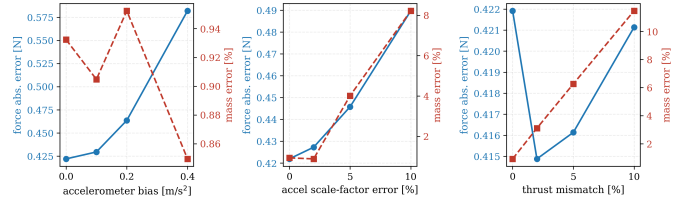
Fig. 13. Robustness to real-sensor errors. Force absolute error (blue, left axis) and mass calibration error (red, right axis) against injected accelerometer bias, accelerometer scale-factor error, and thrust-coefficient mismatch. The virtual sensor degrades gracefully and proportionally, with no catastrophic failure.
