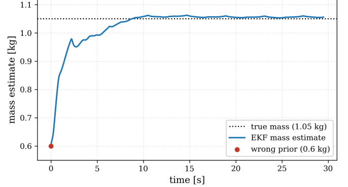
Fig. 5. Mass identification under excitation. From a wrong prior (0.60 kg) the EKF converges to within 0.6 % of the ground truth on a disturbance-free trajectory.
