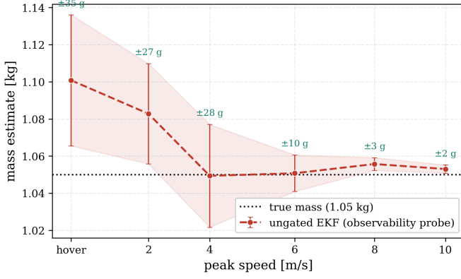
Fig. 6. Mass observability against excitation, probed with an ungated EKF ( N=10 per speed, N=9 in hover; mean \pm std): biased in hover, accurate under excitation, confirming Proposition 1 and the \sigma^{-1} conditioning.
