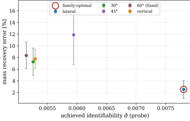
Fig. 9. Probe shaping by identifiability. Sweeping the probe’s vertical/lateral mix at a fixed displacement budget, the mass recovery error falls as \tilde{\sigma} rises; the \tilde{\sigma} -maximizing mix is circled.
