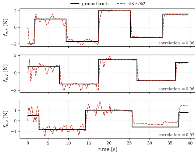
FIGURE 2. Virtual force sensor in the time domain (representative run): \hat{m}\hat{\mathbf{a}} tracks the applied wind steps on all three axes.
