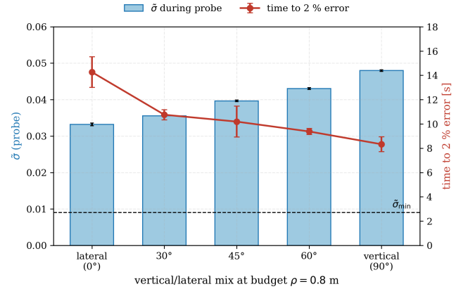
FIGURE 9. Probe shaping at the 0.8 m budget: identifiability achieved while the probe is active (bars) and time for the mass error to settle below 2 % (line), against the vertical/lateral mix ( N=5 per shape, mean \pm std).
