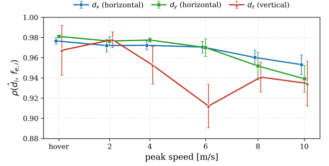
FIGURE 3. Per-axis force correlation against excitation ( N=10 ; 9 in hover; step ground truth).
