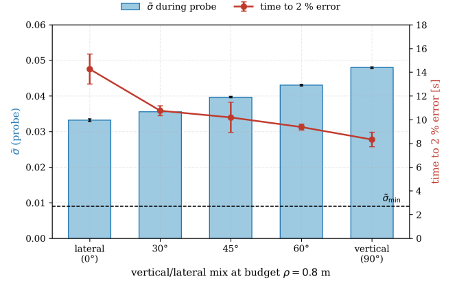
FIGURE 9. Probe shaping at the 0.8 m budget: identifiability achieved while the probe is active (bars) and time for the mass error to settle below 2% (line), against the vertical/lateral mix ( N=5 per shape, mean \pm std).
