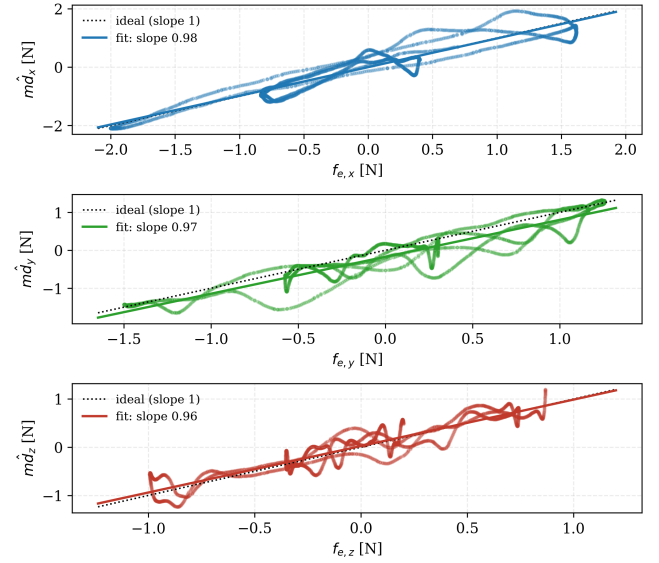
FIGURE 4. Calibration curve under a sinusoidal wind: estimated force against applied force for, from top to bottom, the x, y, and z axes, with the linear fit (slopes 0.98, 0.97, 0.96; R^2 0.90, 0.89, 0.87) and the ideal unit slope.
