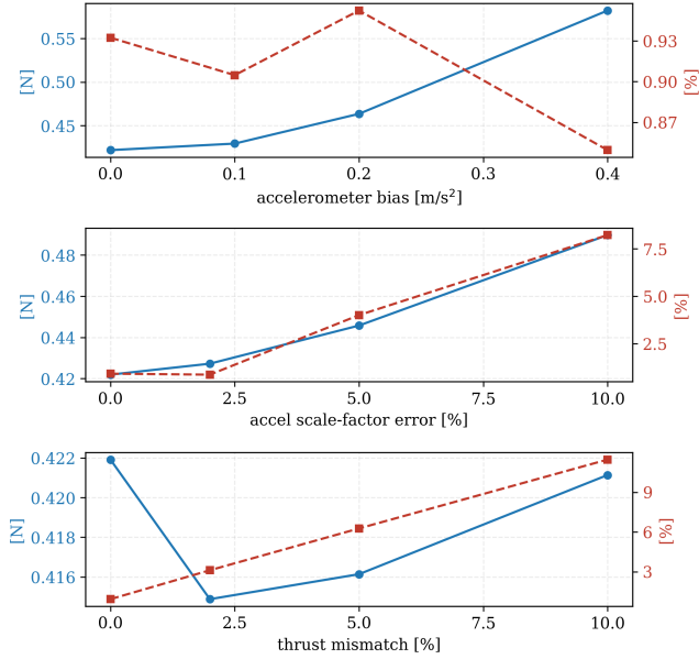
FIGURE 13. Robustness to injected accelerometer bias, scale-factor error, and thrust mismatch: force error (blue, left axis) and mass error (red, right axis).
