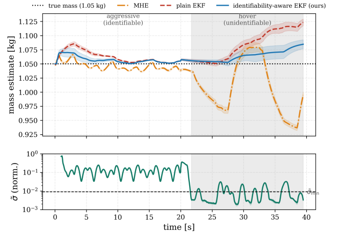
FIGURE 7. Mass over a windy maneuver-to-hover transition ( N=5 , mean \pm std); hover shaded, identifiability signal and threshold at the bottom.
