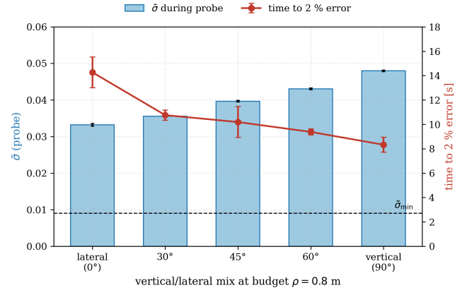
FIGURE 9. Probe shaping at the 0.8 m budget: identifiability achieved while the probe is active (bars) and time for the mass error to settle below 2 % (line), against the vertical/lateral mix ( N=5 per shape, mean \pm std).
