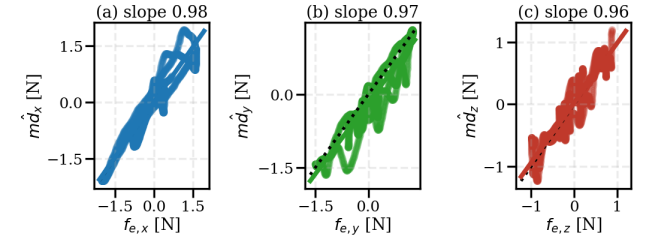
FIGURE 4. Calibration curve under a sinusoidal wind: estimated force against applied force for the (a) x , (b) y , and (c) z axes, with the linear fit (slopes 0.98, 0.97, 0.96 ; R^2 0.90, 0.89, 0.87 ) and the ideal unit slope.
