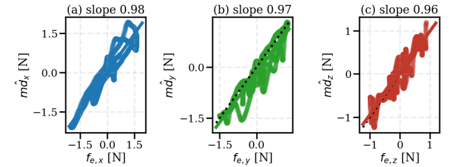
FIGURE 4. Calibration curve under a sinusoidal wind: estimated force against applied force for the (a) x, (b) y, and (c) z axes, with the linear fit (slopes 0.98, 0.97, 0.96; R^2 0.90, 0.89, 0.87) and the ideal unit slope.
