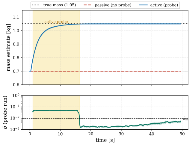
FIGURE 8. Mass recovery from a wrong hover prior (0.70 kg; wind-free hover; N=5 , mean \pm std): the probe (shaded) lifts \sigma , recovers the mass, and is withdrawn after 15 s of gate-open time; the estimate is then held for the rest of the hover.
