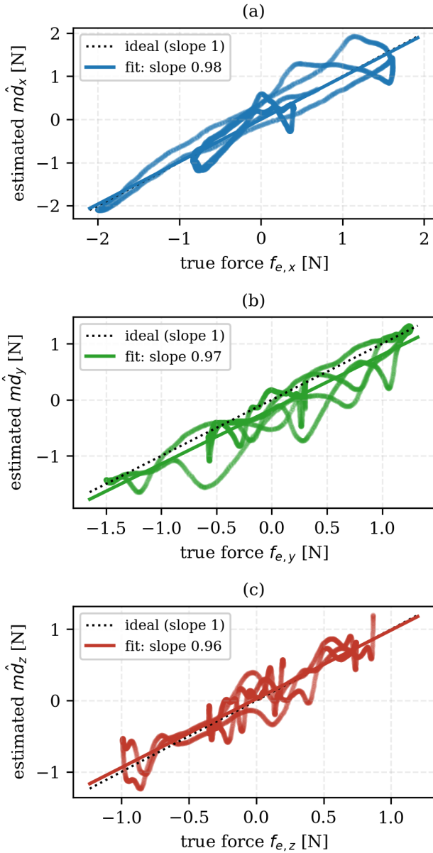
FIGURE 4. Calibration curve under a sinusoidal wind: estimated force against applied force for the (a) x , (b) y , and (c) z axes, with the linear fit (slopes 0.98, 0.97, 0.96; R^2 0.90, 0.89, 0.87) and the ideal unit slope.
