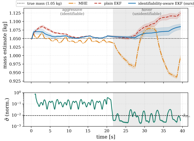
FIGURE 7. Mass over a windy maneuver-to-hover transition ( N=5 , mean \pm std); hover shaded, \sigma and threshold at the bottom.
