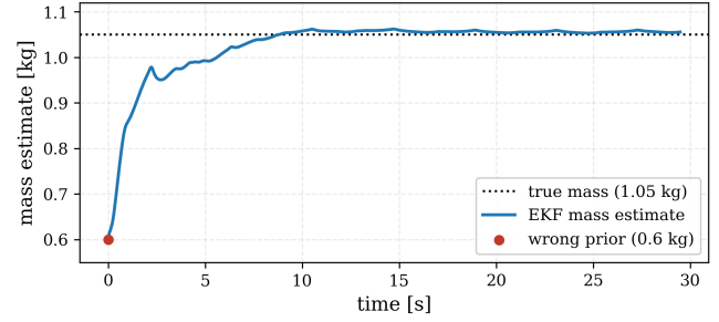
FIGURE 5. Mass identification under excitation: from a 0.60 kg prior to within 0.6% (disturbance-free trajectory).
