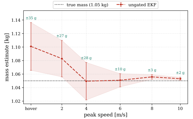
FIGURE 6. Mass identifiability against excitation, ungated EKF ( N=10 per speed, N=9 in hover; mean \pm std).
