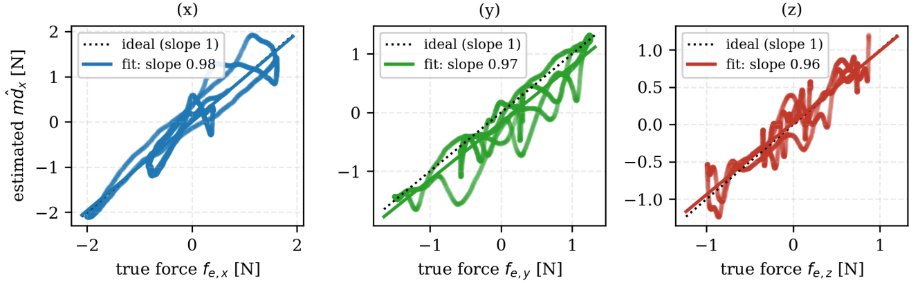
FIGURE 4. Calibration curve under a sinusoidal wind: estimated force against applied force for the (a) x , (b) y , and (c) z axes, with the linear fit (slopes 0.98, 0.97, 0.96; R^2 0.90, 0.89, 0.87) and the ideal unit slope.
