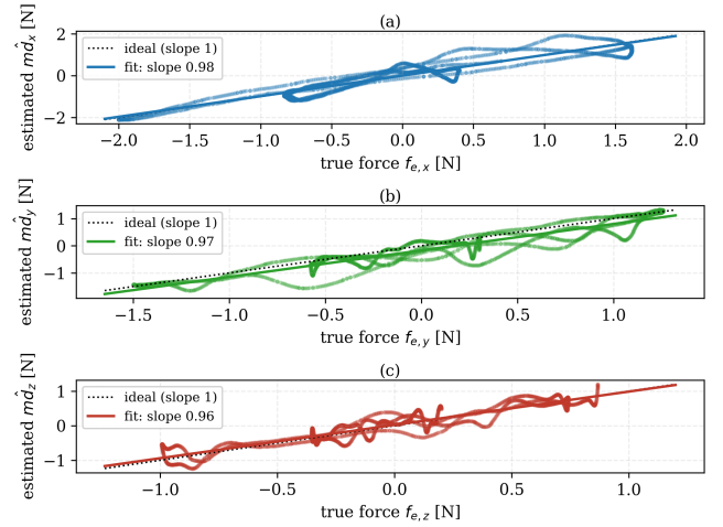
FIGURE 4. Calibration curve under a sinusoidal wind: estimated force against applied force for the (a) x , (b) y , and (c) z axes, with the linear fit (slopes 0.98, 0.97, 0.96; R^2 0.90, 0.89, 0.87) and the ideal unit slope.
