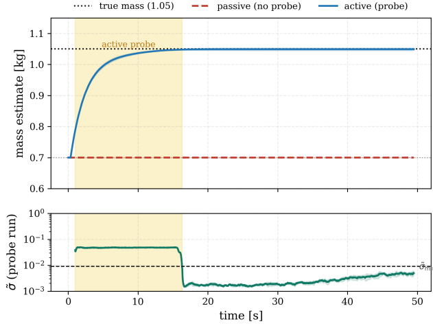
FIGURE 8. Mass recovery from a wrong prior (0.70 kg) in wind-free hover ( N=5 , mean \pm std): the probe (shaded) lifts \sigma and recovers the mass, is withdrawn after 15 s of gate-open time, and the estimate holds for the rest of the hover. Unlike the excited trajectory of Fig. 5, hover provides no information: the passive filter stays at the prior.
