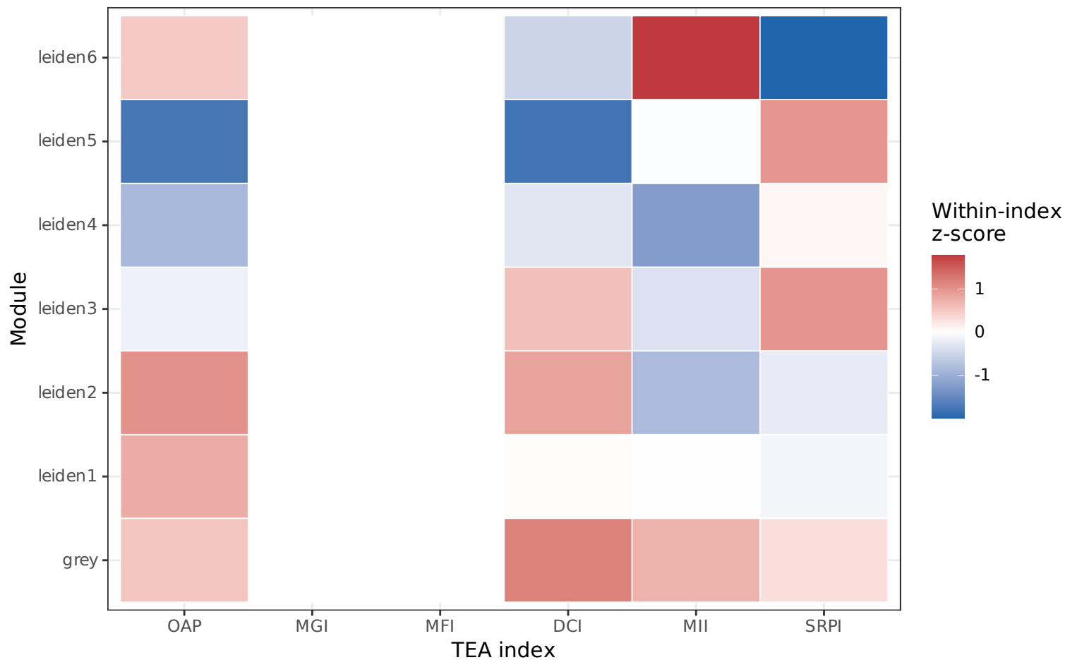
Module-level TEA central tendency (raw, scaled within index) Z-score of module medians within each index (relative enrichment/depletion)
