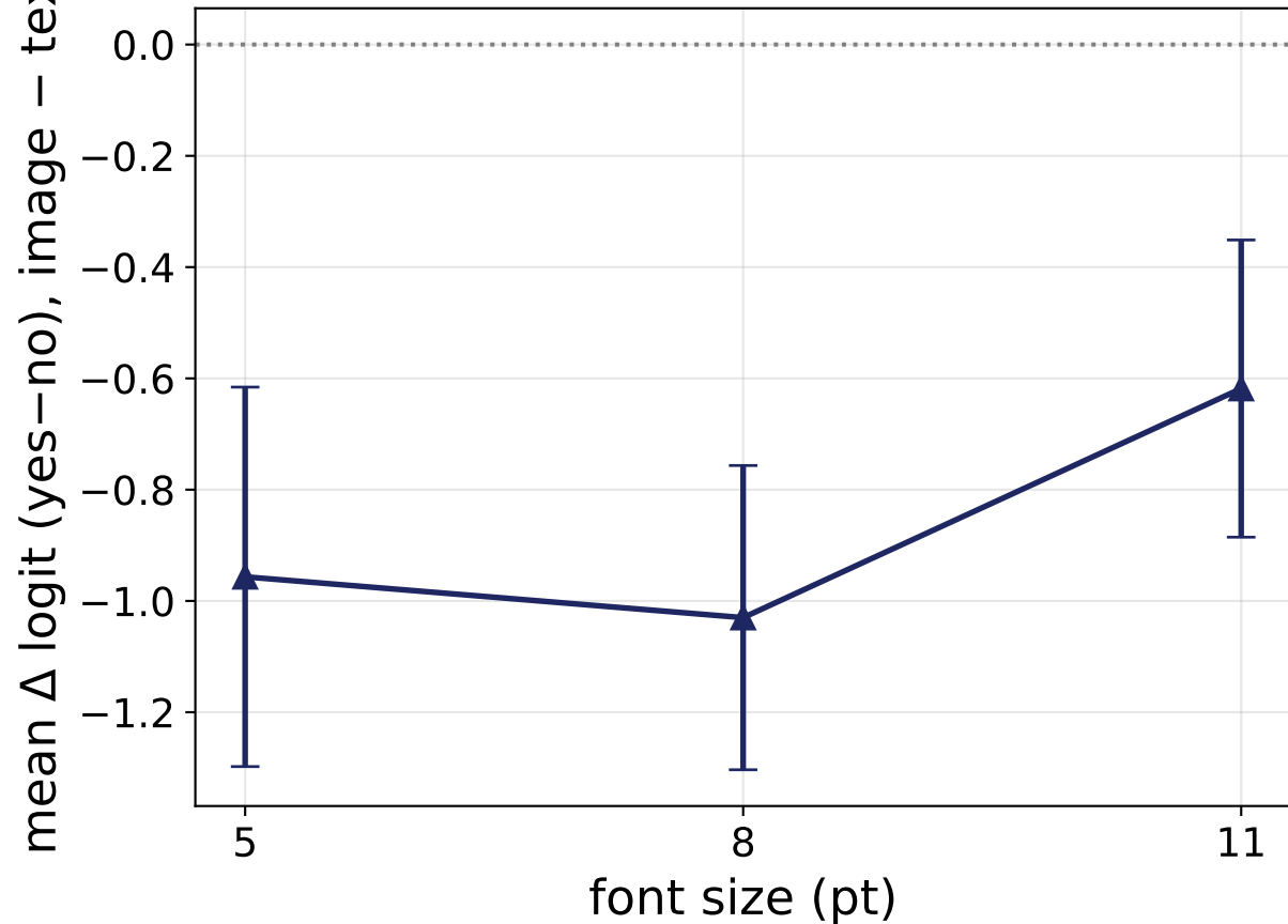
Directional bias vs render size (95% CI)
