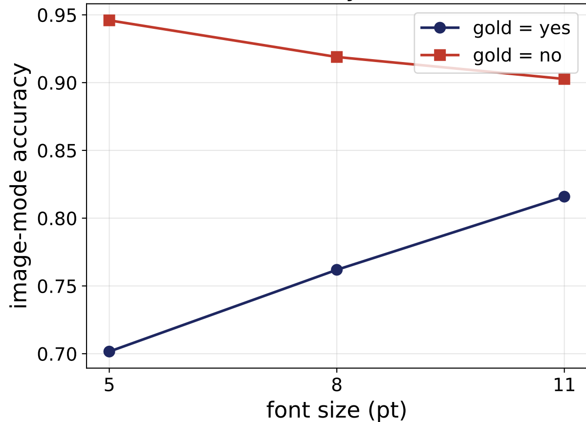
Per-class accuracy vs render size
