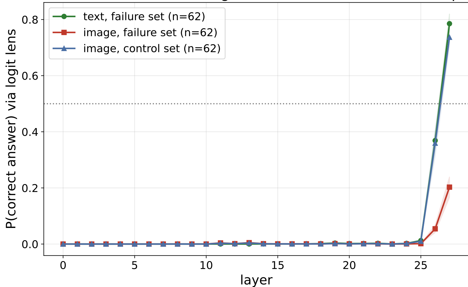
Where the answer emerges — Qwen2.5-VL-7B, BoolQ, 5pt
