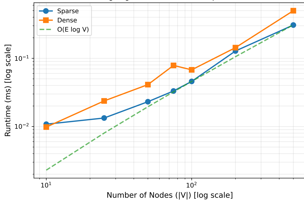
Log-Log Plot: Runtime vs. Graph Size
