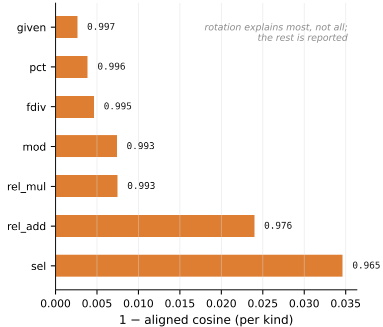
what did not align — residual 0.155
