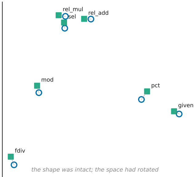
after orthogonal Procrustes — mean cos 0.988
