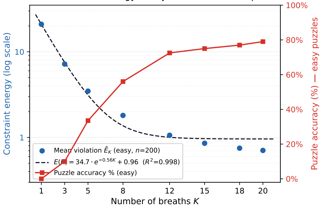
Constraint energy decay — Sudoku K-sweep
