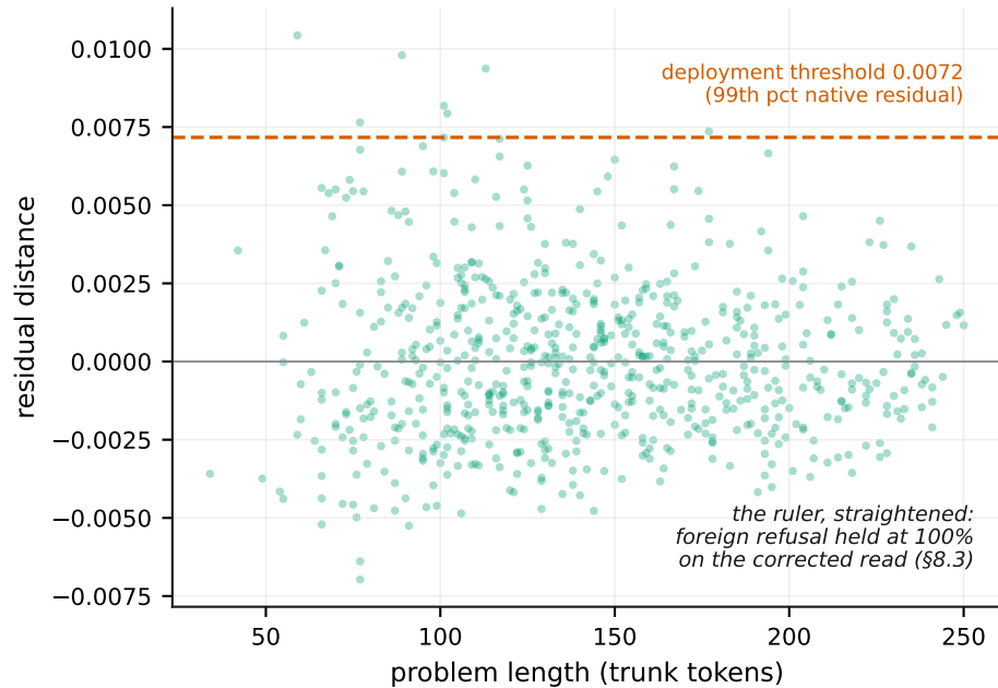
length-controlled residual — r = -0.024
