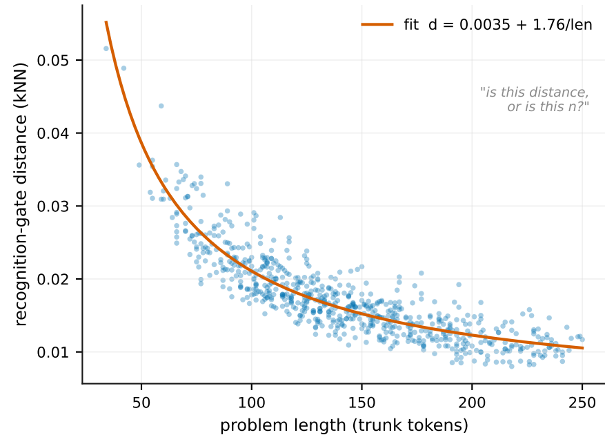
raw distance — r = -0.825 with length
