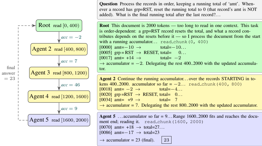
Figure 2: Sequential fold , for order-dependent tasks (variable tracking, running state). Each agent reads the next slice, updates the accumulator, and delegates the rest of the document to the next agent.
