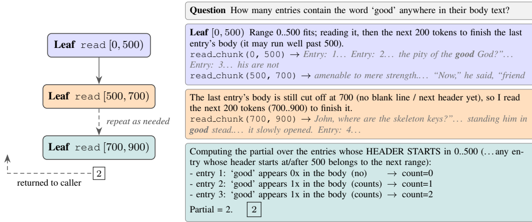
Figure 3: Boundary handling. A leaf/fold agent owns the records whose first line starts in its range. It reads its range plus the next 200 tokens; while its last owned record is still cut off, it reads 200 more (dashed).
