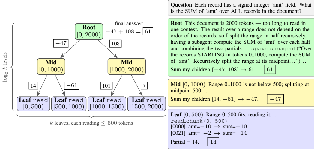
178 179 180 181 182 183 184 185 186 187 188 189 190 191 192 193 194 195 196 197 198 199 200 201 202 203 204 Figure 1: Tree reduce , for order-independent tasks (aggregation, retrieval). Non-leaf nodes delegate half their range to subagents. Leaves read one chunk and compute a leaf op which is aggregated up the tree.
