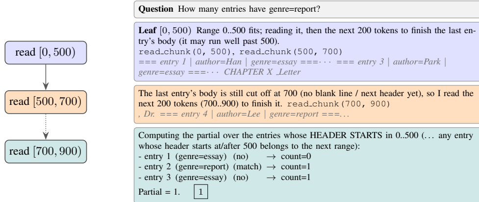
Figure 3: Boundary handling. A leaf owns the records whose first line starts in its range. It reads its range plus the next 200 tokens; while its last owned record is still cut off, it reads 200 more (dotted). Entry 3 starts before 500 but runs past 700, so the leaf reads to 900, where entry 4’s header appears. Entry 4 starts at or after 500, so it belongs to the next leaf and is not counted here.
