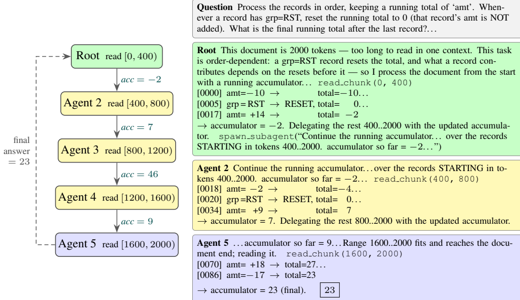
Figure 2: Sequential fold , for order-dependent tasks (variable tracking, running state). Each agent reads the next slice, updates the accumulator, and delegates the rest of the document to the next agent.
