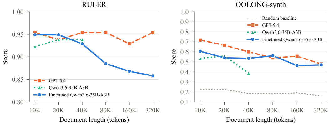
Figure 1: Results on RULER and OOLONG-synth. Our finetune runs in our harness with an 8K token per-agent context limit. GPT-5.4 (medium reasoning) and base Qwen3.6-35B-A3B (thinking disabled) receive the full document with the prompt (see Section 4 and Appendix A for more details). Base Qwen and GPT-5.4 are served with 64K and 1M token context limits, respectively. The OOLONG random baseline follows Bertsch et al. (2025, §2.3).
