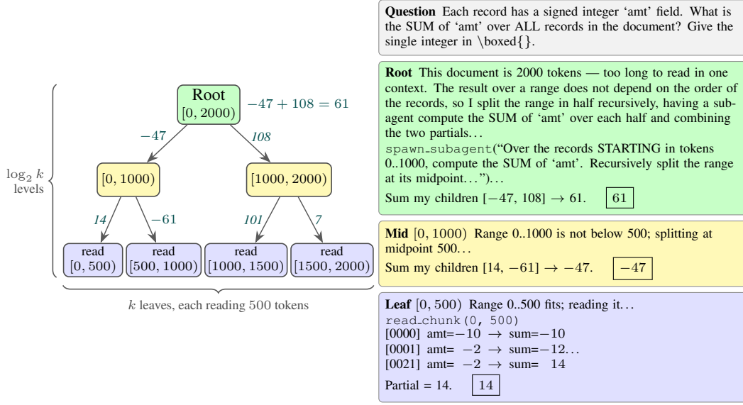
Figure 1: Tree reduce , for order-independent tasks (aggregation, retrieval). Non-leaf nodes delegate half their range to subagents. Leaves read one chunk and compute a leaf op which is aggregated up the tree.
