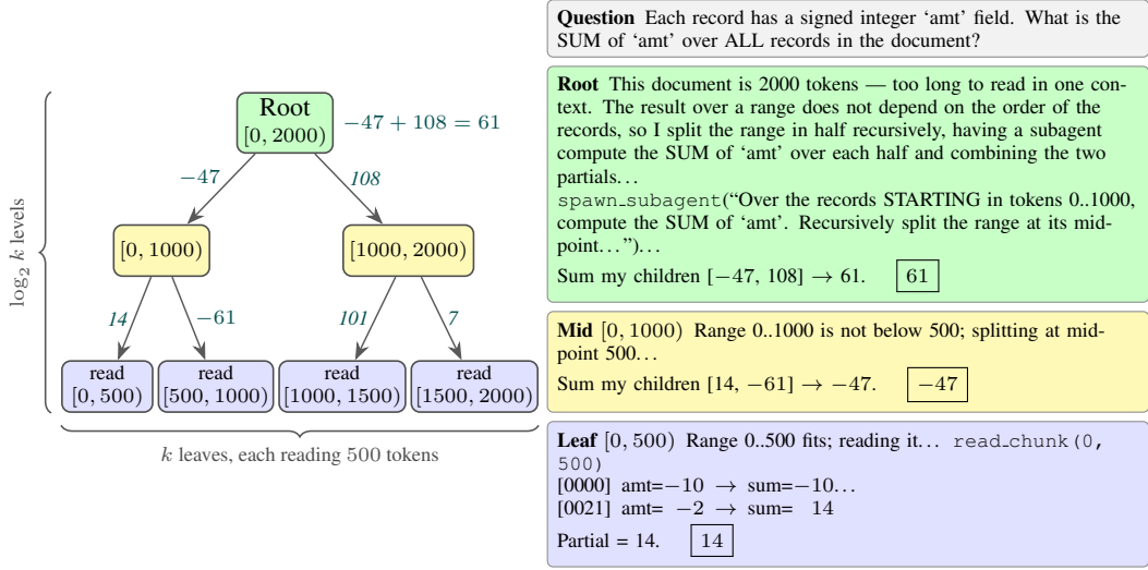
Figure 1: Tree reduce , for order-independent tasks (aggregation, retrieval). Non-leaf nodes delegate half their range to subagents. Leaves read one chunk and compute a leaf op which is aggregated up the tree.
